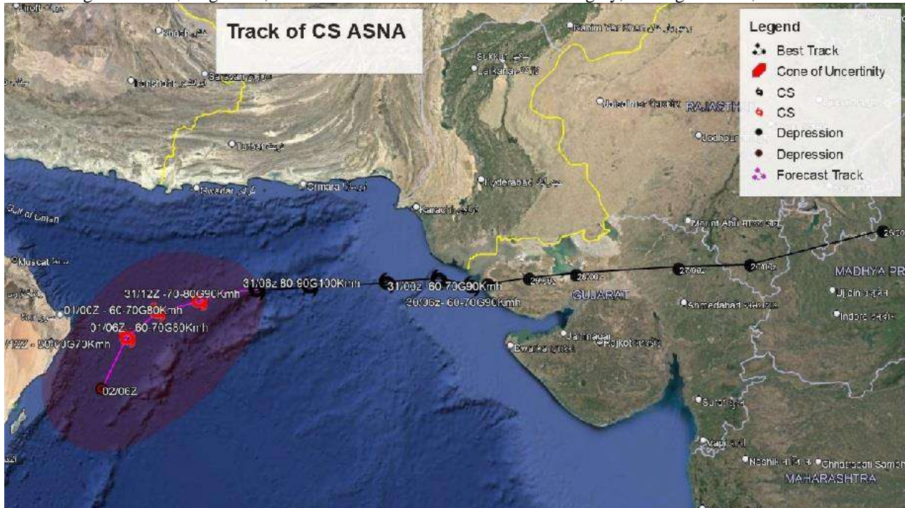
Observed & Forecast Track
