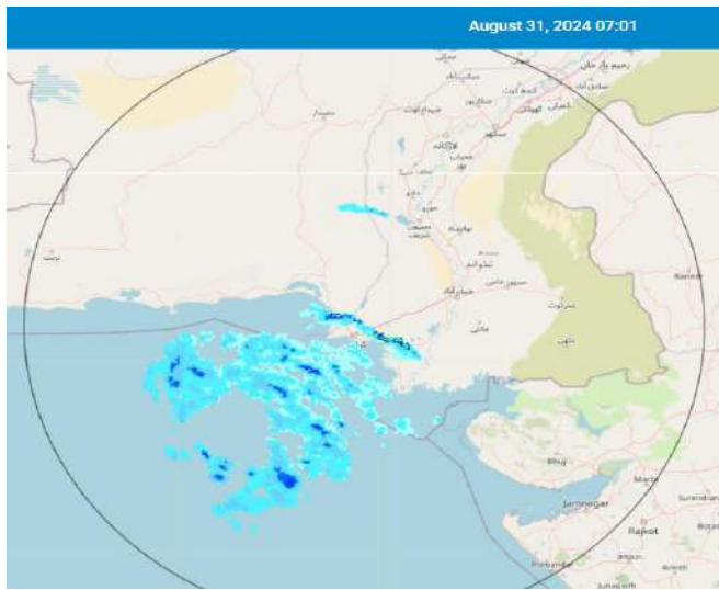
Radar Image 0700PST, August 31, 2024
